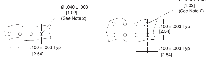
Recommended Mounting Hole Pattern
